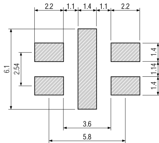
Figure 3) Land Pattern
