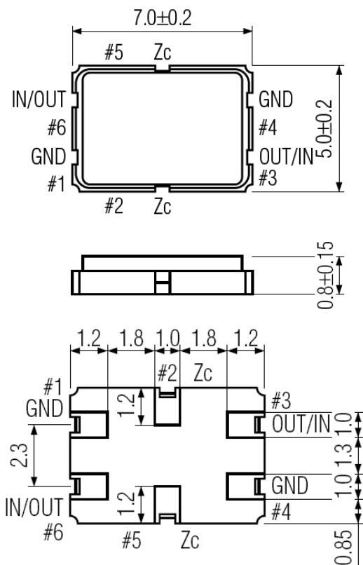
Figure 1) Top, Side and Bottom Views
