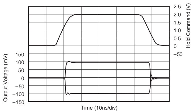
SOTA HOLD COMMAND DELAY TIME
