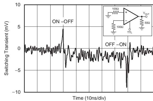
SOTA SWITCHING TRANSIENTS
