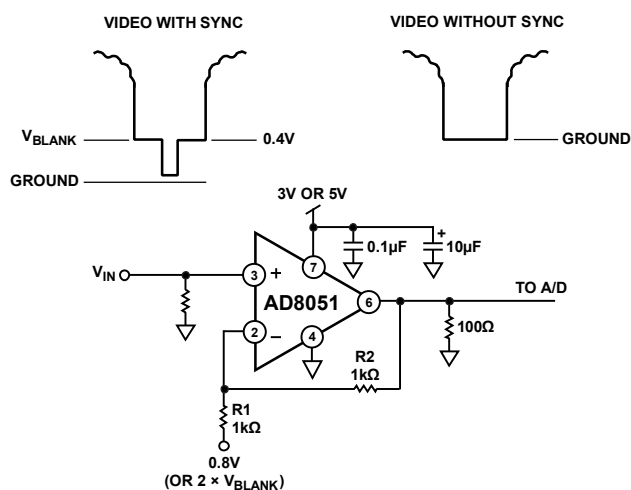
Figure 51. Sync Stripper
