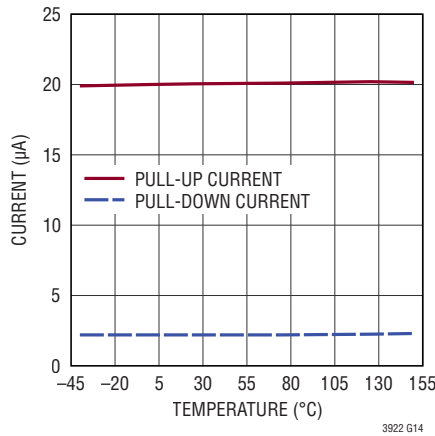
SS Currents
