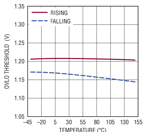
OVLO Threshold
