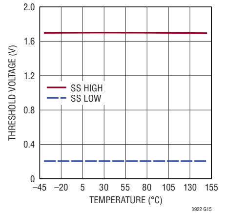
SS Thresholds
