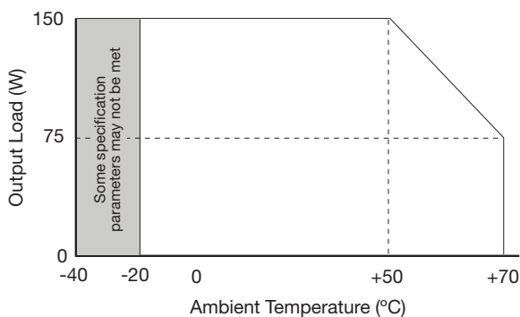
Figure 5 - 150 W Convection Cooled
