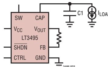
Figure 3. Improved Efficiency Connection
