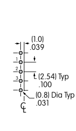
B1 Terminals
