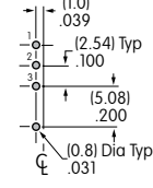
V1 Terminals
