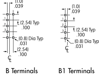
A12K1B-DA
