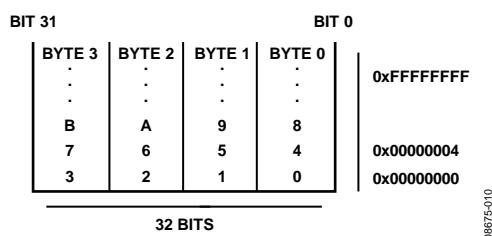
Figure 16. Little Endian Format
