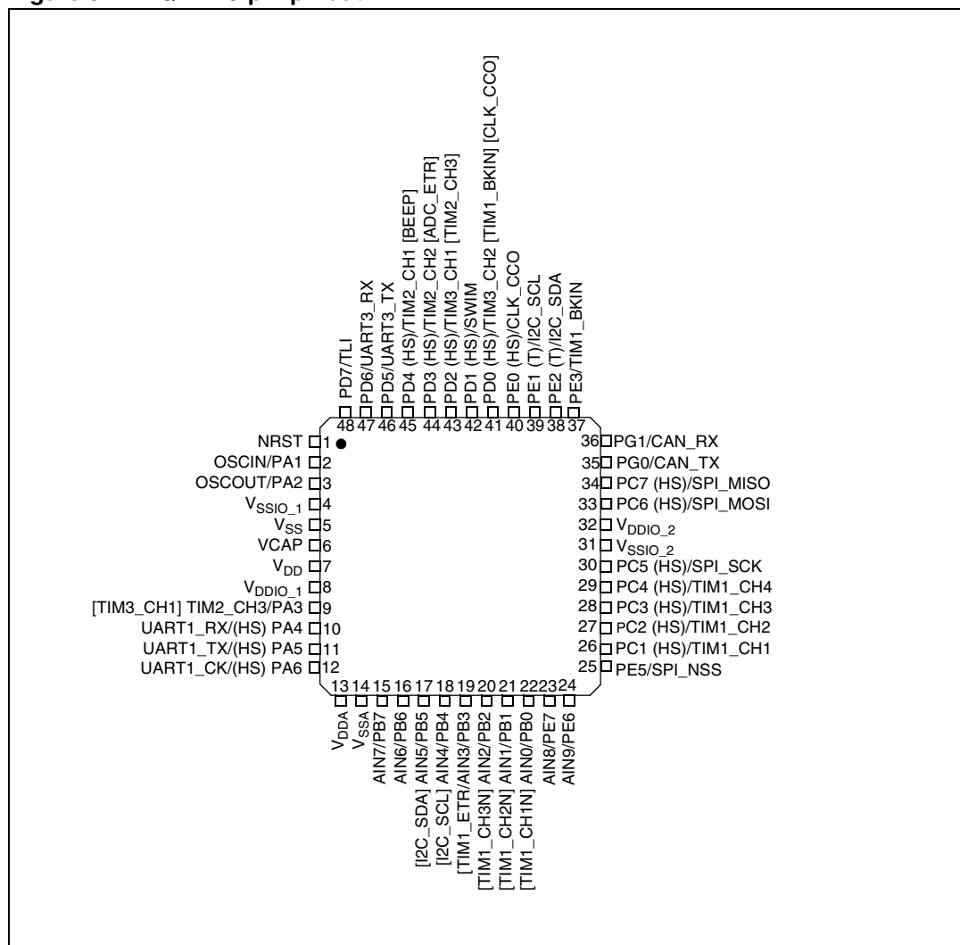
Figure 5. LQFP 48-pin pinout
