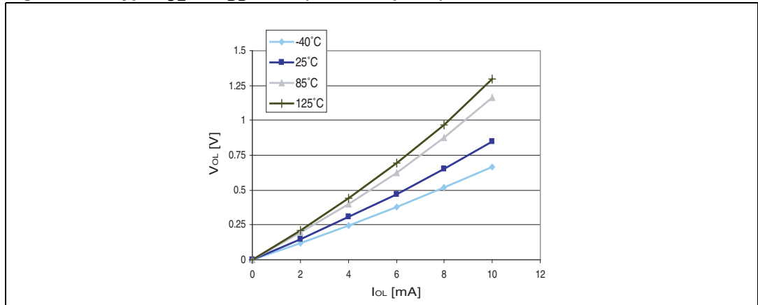
Figure 23. Typ. V_{OL} @ V_{DD} = 5\text{ V} (standard ports)
