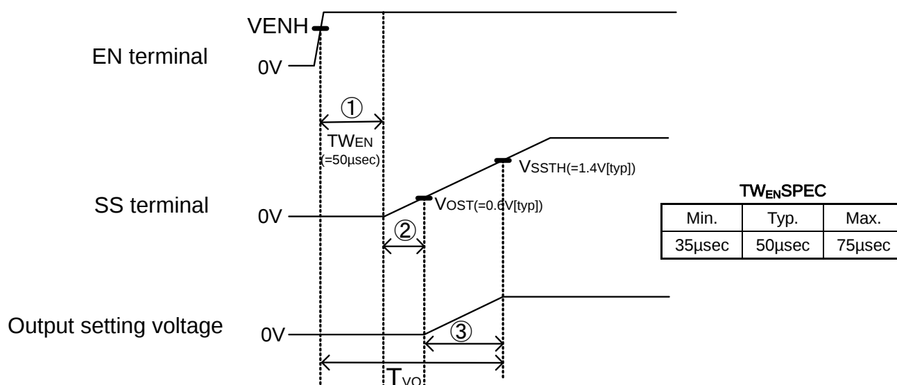
Fig.17 Soft start
