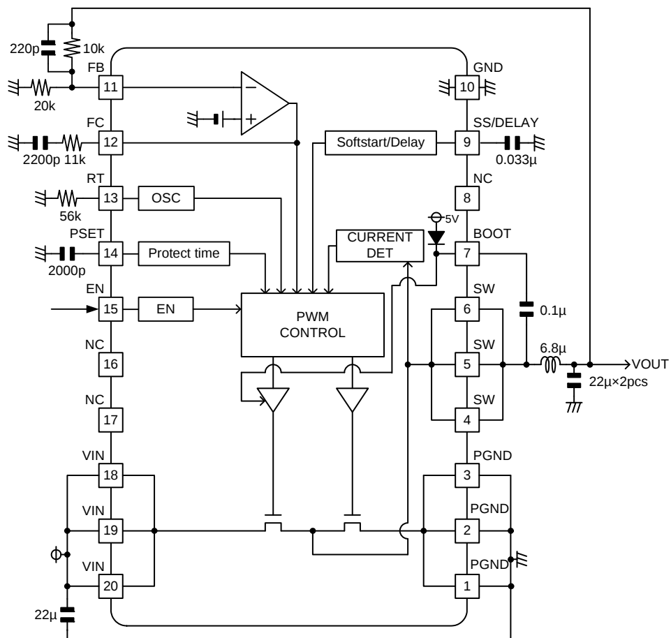
Fig.20 Typical application
