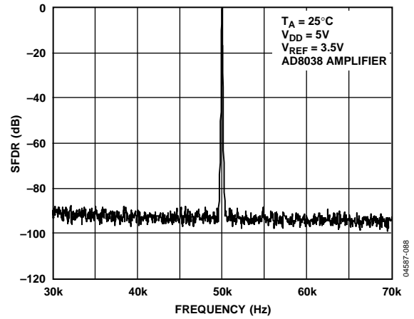
Figure 39. Narrow-Band SFDR, f_{OUT} = 50 kHz, Clock = 1 MHz
