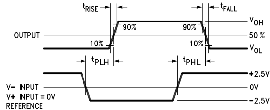
Figure 3. Propagation Delay
