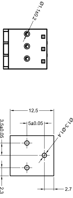
PCB Layout
