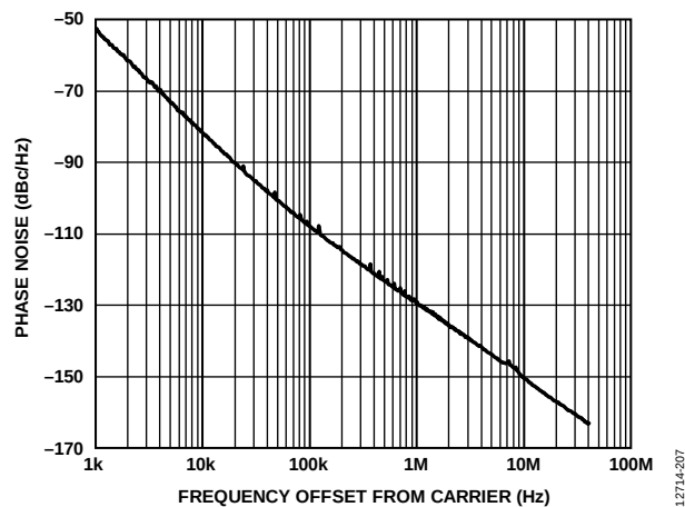
Figure 7. Open-Loop VCO Phase Noise, 8.0 GHz
