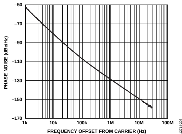
Figure 8. Open-Loop VCO Phase Noise, 10.0 GHz
