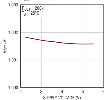
V_{SET} vs Supply Voltage
