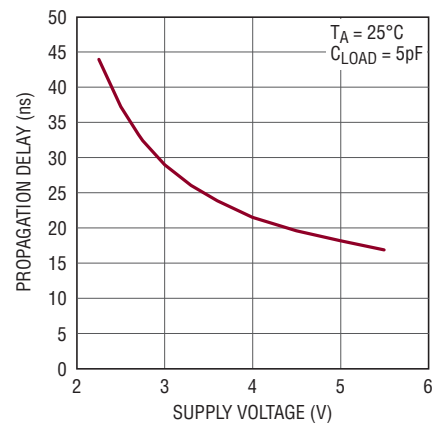
Output Disable Propagation Delay ( t_{PD} ) vs Supply Voltage
