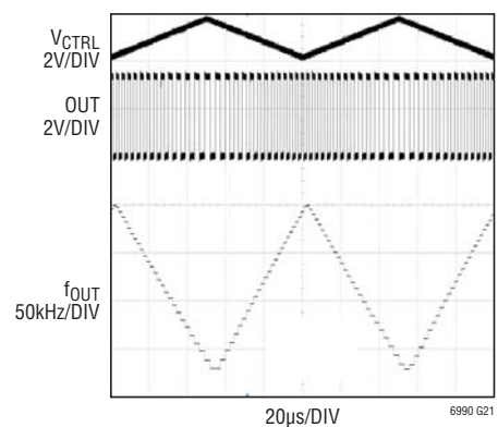
Frequency Modulation
