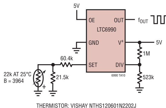
Temperature to Frequency Converter. 3% Linearity from -20^{\circ}\text{C} ( f_{\text{OUT}} \approx 20\text{kHz} ) to 75^{\circ}\text{C} ( f_{\text{OUT}} \approx 25\text{kHz} )
