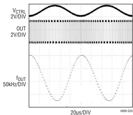
Frequency Modulation
