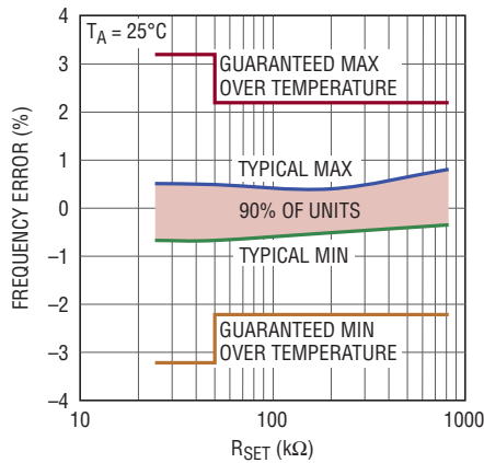
Frequency Error vs R_{SET}
