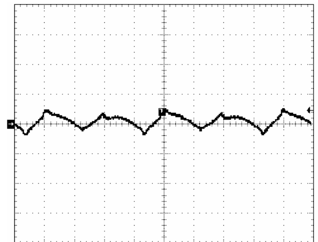
Fig.1.8V-7: Output voltage ripple (50mV/div) at full rated load current into a resistive load with Co=10µF tantalum + 1µF ceramic and Vin=48V. Time scale: 1µs/div
