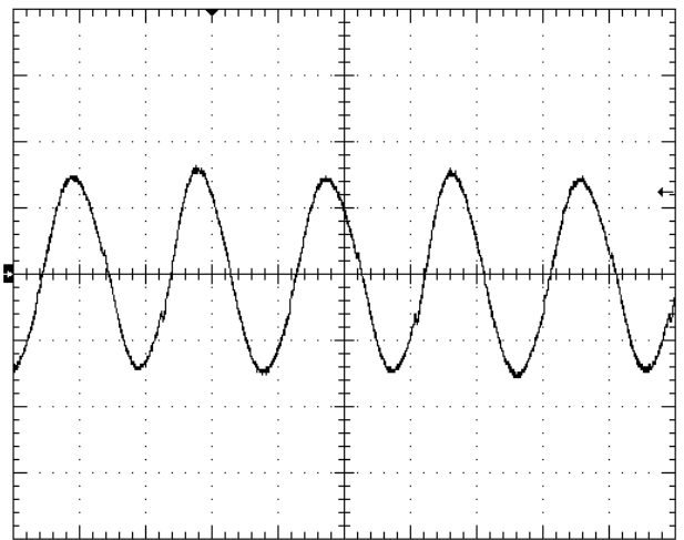
Fig.2.5V-10: Input reflected ripple current, I_c (100mA/div), measured through 10µH at the source at full rated load current and V_{in}=48V . Time scale: 1µs/div.
