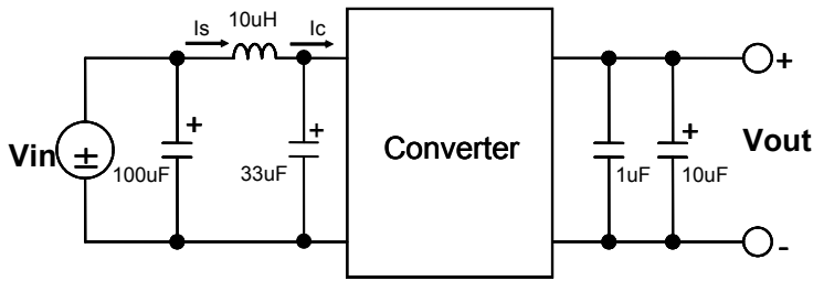
Fig.2.5V-8: Test Set-up for measuring input reflected current.
