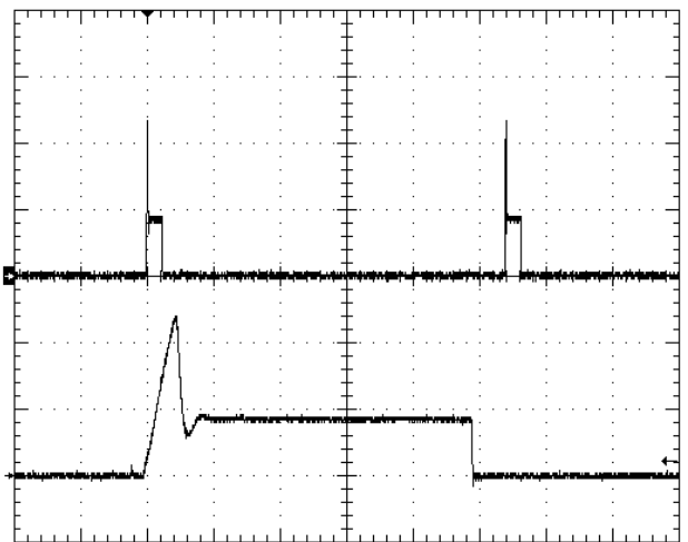
Fig.2.5V-12: Load current (top trace, 50A/div, 40ms/div) into a 10mΩ short circuit during restart, at V_{in} = 48V . Bottom trace (50A/div, 2ms/div) is an expansion of the top trace.
