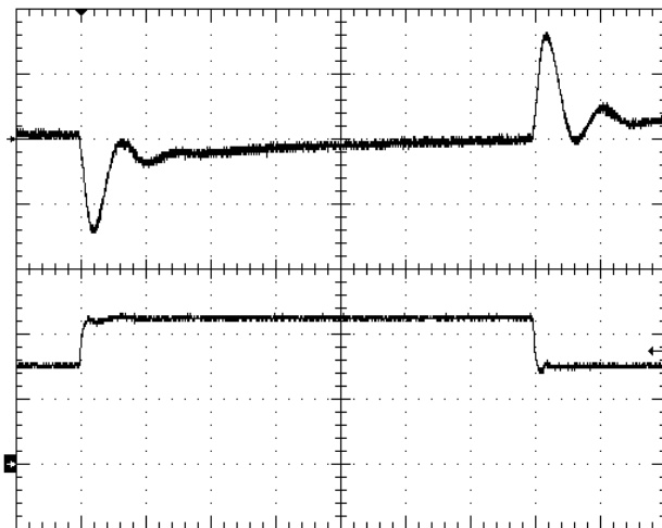
Fig.1.5V-6: Output voltage response to load current step-change (15 \leftrightarrow 22.5A) at Vin=48V. Top trace: Output voltage (100mV/div). Bottom trace: load current (10A/div). Current slew rate: 5A/ \mu s. Co=470 \mu F os-con + 10 \mu F tantalum + 1 \mu F ceramic. Time scale: 100 \mu s/div
