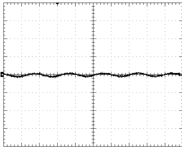
Fig.2.5V-9: Input reflected ripple current, I_s (5mA/div), measured through 10µH at the source at full rated load current and V_{in}=48V . Time scale: 1µs/div.
