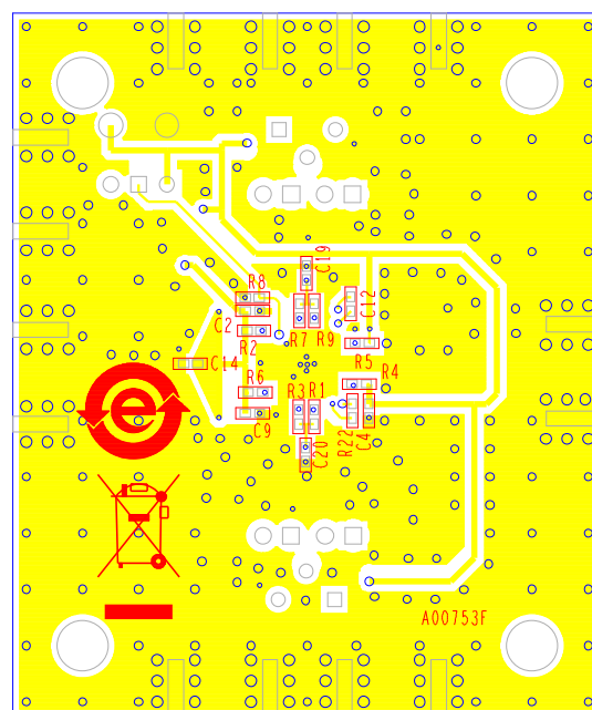
Figure 43. AD8341 Evaluation Board Bottom Layer
