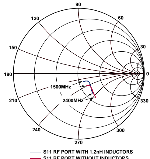
Figure 20. Input Impedance Smith Chart
