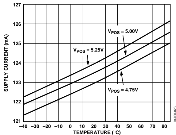
Figure 23. Supply Current vs. Temperature
