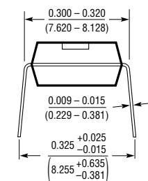
N8 Package 8-Lead Plastic DIP
