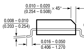
S8 Package 8-Lead Plastic SOIC
