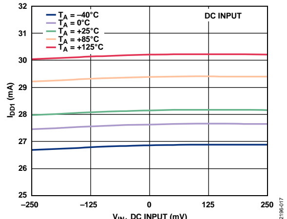
Figure 23. ID1 vs. VIN+ DC Input at Various Temperatures
