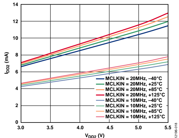
Figure 24. ID2 vs. VDD2 at Various Temperatures and Clock Rates
