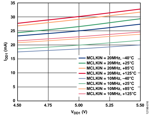
Figure 22. ID1 vs. VDD1 at Various Temperatures and Clock Rates
