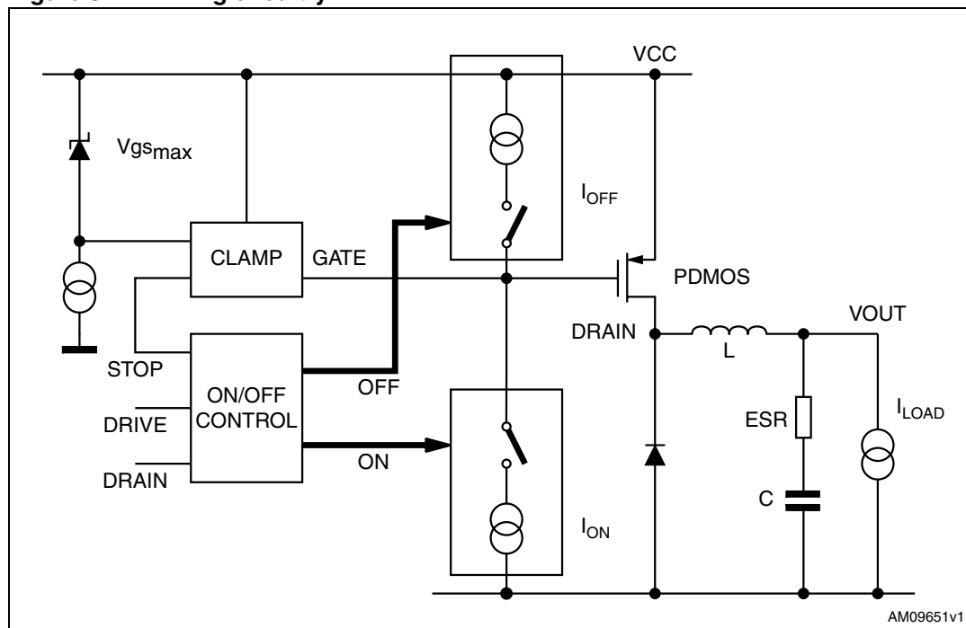
Figure 8. Driving circuitry
