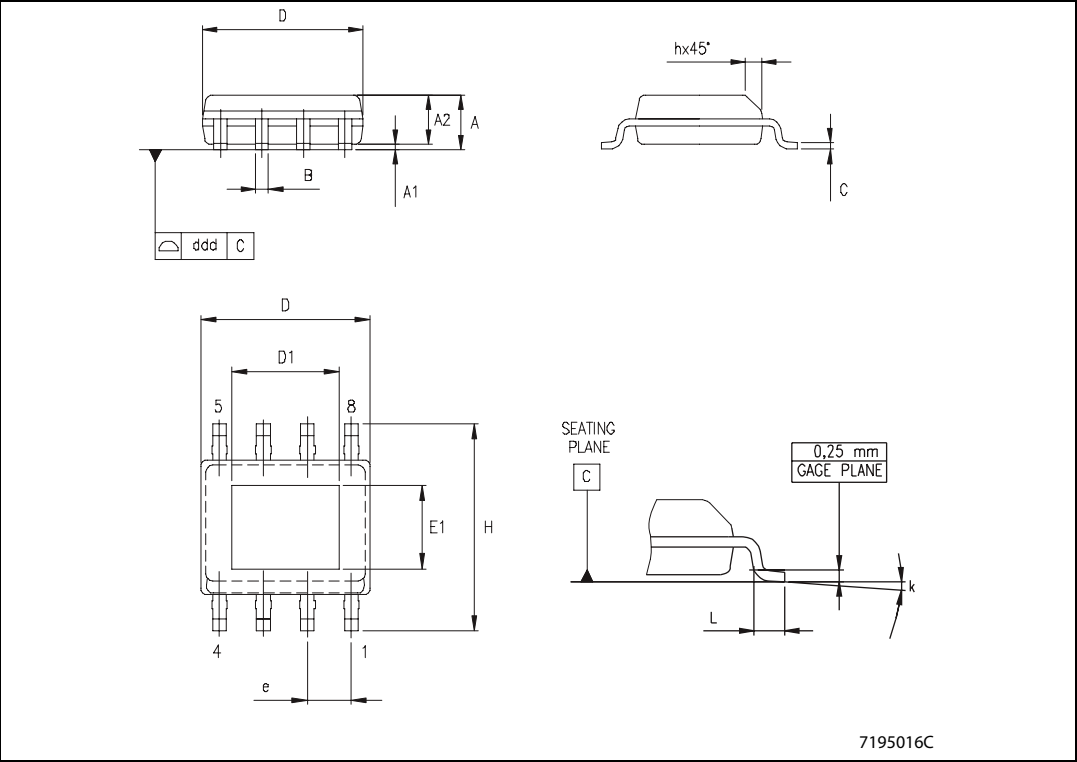
Figure 42. Package dimensions
