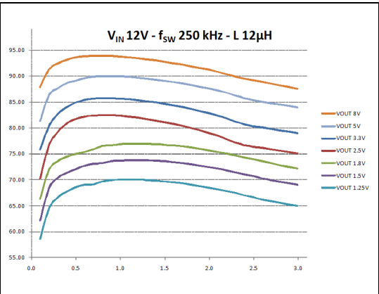
Figure 40. Efficiency vs. output current ( V_{IN} 12 V)
