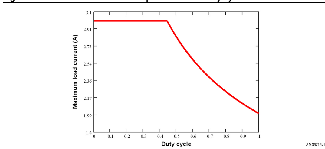
Figure 18. Maximum continuous output current vs. duty cycle
