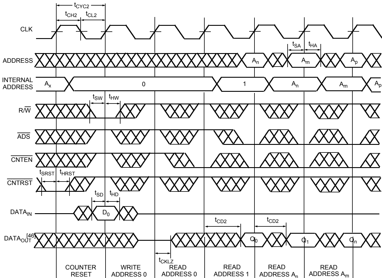
Figure 12. Counter Reset [44, 45]
