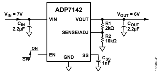
Figure 43. Typical Adjustable Output Voltage Application Schematic
