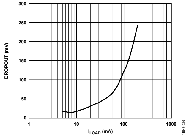
Figure 22. Dropout Voltage vs. Load Current ( I_{LOAD} ), V_{OUT} = 3.3 V
