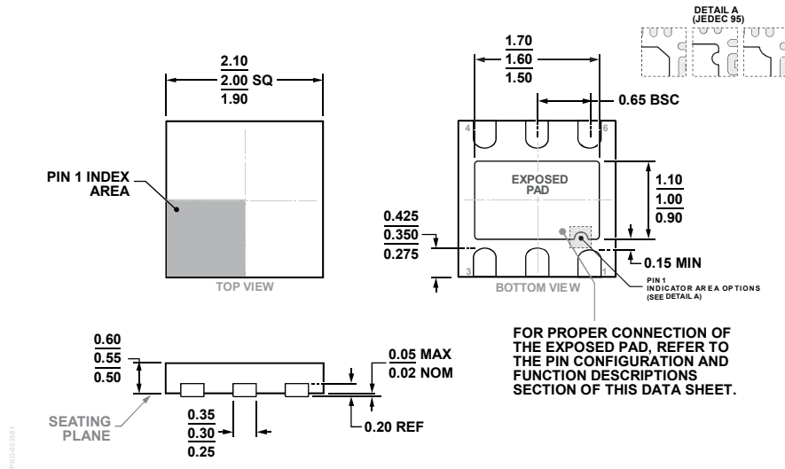
Figure 67. 6-Lead Lead Frame Chip Scale Package [LFCSP] 2.00 mm × 2.00 mm Body and 0.55 mm Package Height (CP-6-3)
