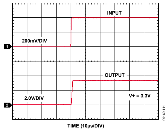
Figure 14. Differential Overload Recovery, Rising ( V^+ = 3.3\text{ V} )
