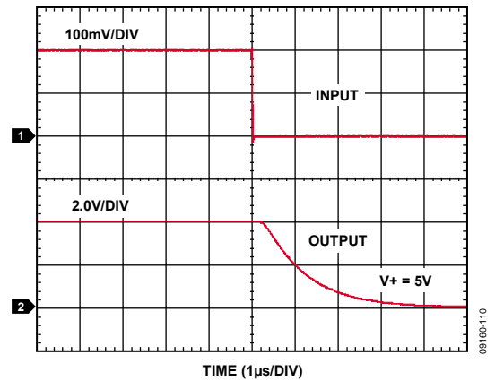
Figure 13. Fall Time ( V^+ = 5\text{ V} )
