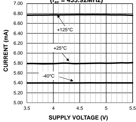
Ground Current vs. Supply Voltage (f RF = 433.92MHz)
