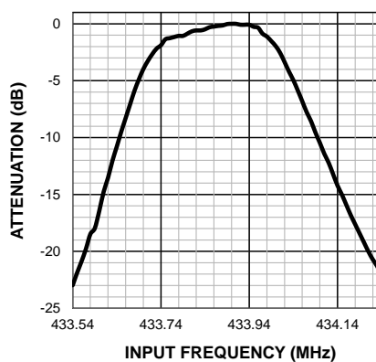
Bandpass Filter Attenuation f XAL = 13.52127MHz
