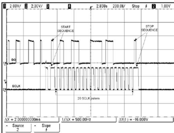
Figure 12. Auto-Poll Example
