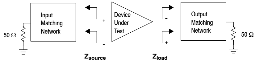
Figure 14. Series Equivalent Source and Load Impedance — 1030 MHz
