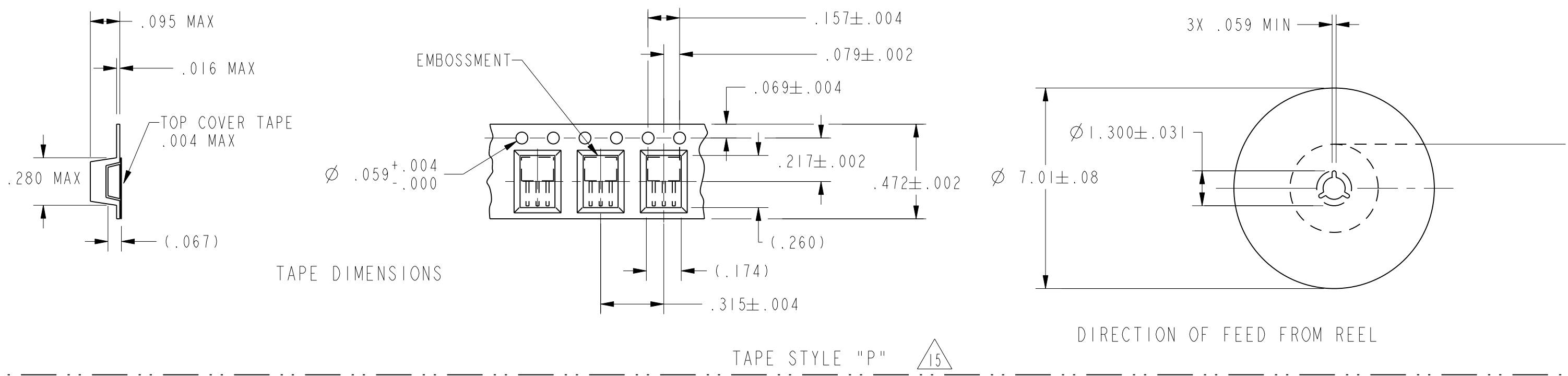
TAPE DIMENSIONS
