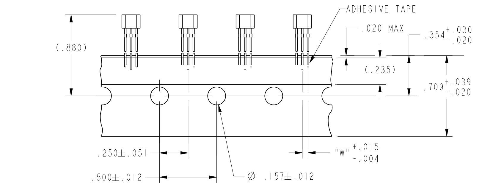
TAPE DIMENSIONS
