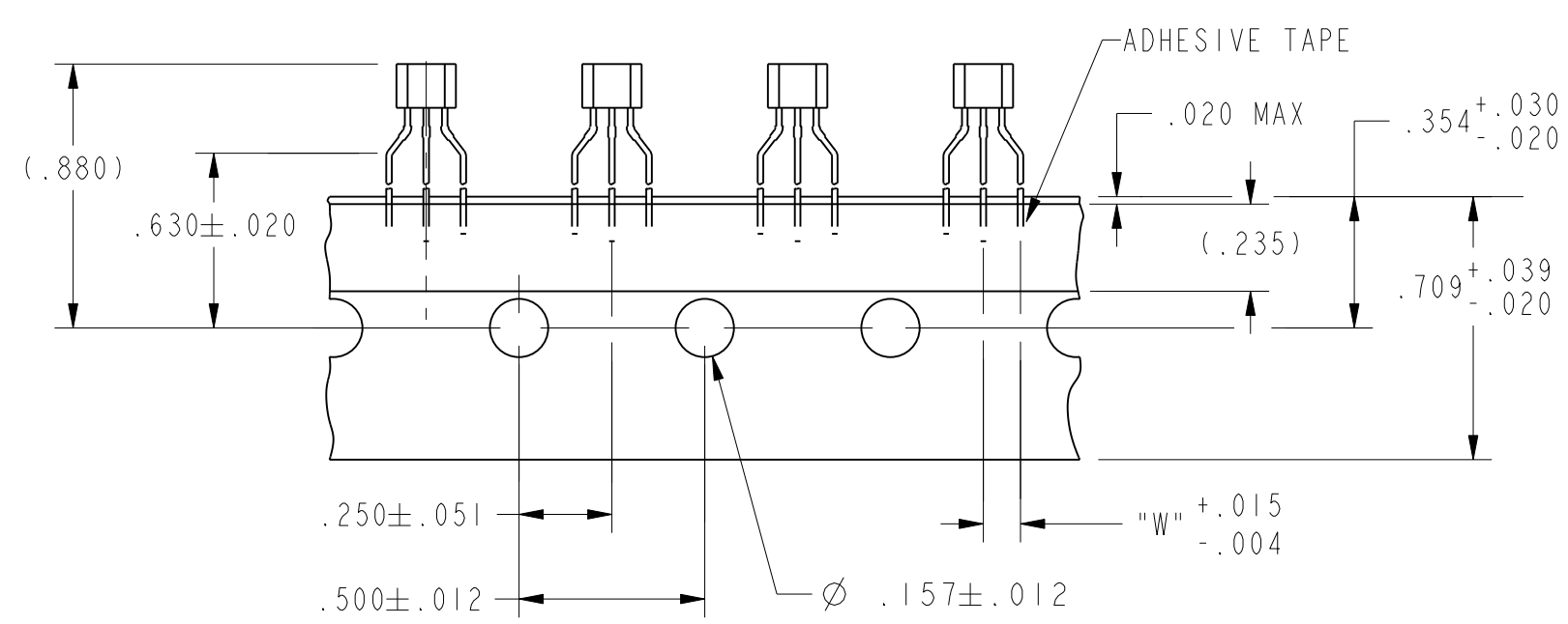
TAPE DIMENSIONS
