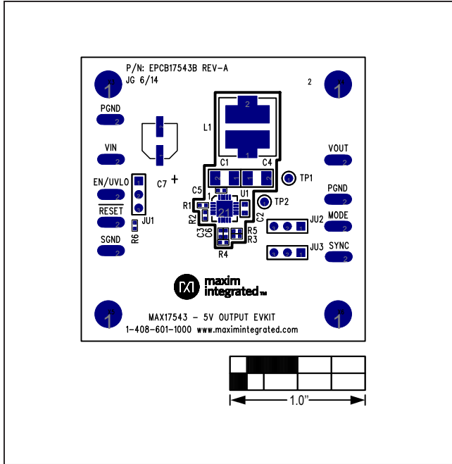
Figure 12. MAX17543 5V Output EV Kit Component Placement Guide—Component Side
