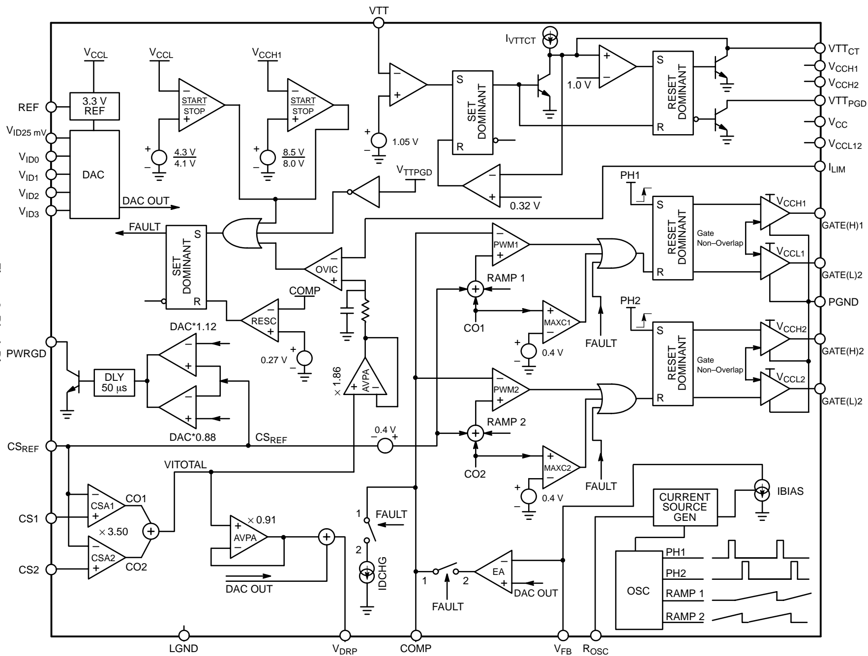
Figure 2. Block Diagram
