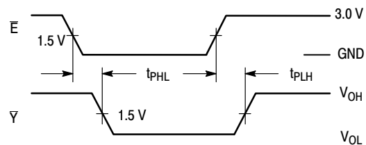
Figure 8. Switching Waveform
