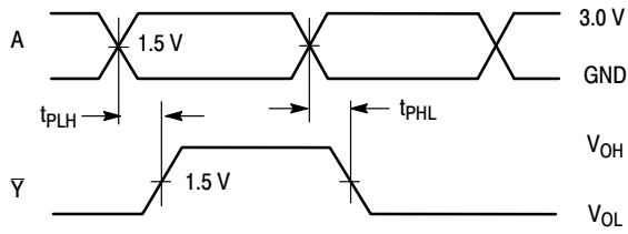
Figure 7. Switching Waveform
