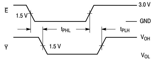
Figure 8. Switching Waveform
