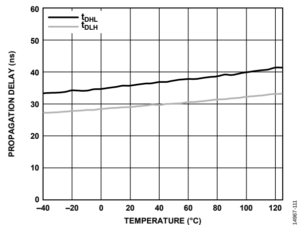
Figure 14. Propagation Delay vs. Temperature, 2 nF Load
