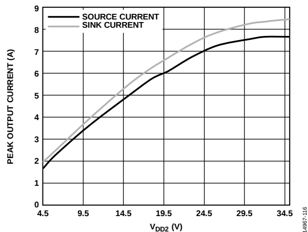
Figure 17. Peak Output Current vs. V_{DD2} , 2 \Omega Series Resistance
