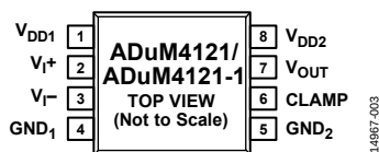
Figure 3. Pin Configuration
