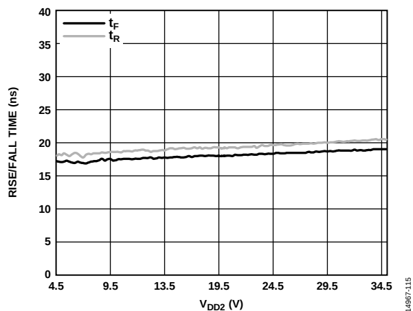
Figure 16. Rise and Fall Time vs. V_{DD2} , 2 nF Load, 3.9 \Omega Resistor
