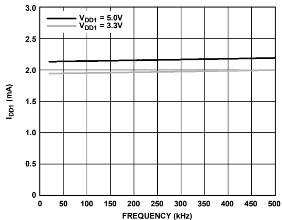
Figure 11. I_{DD1} vs. Frequency
