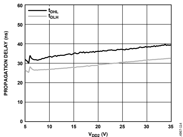
Figure 15. Propagation Delay vs. V_{DD2} , 2 nF Load
