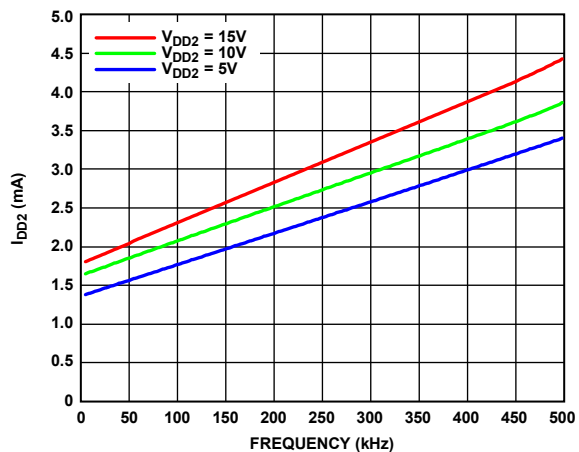
Figure 12. I_{DD2} vs. Frequency with 2 nF Load
