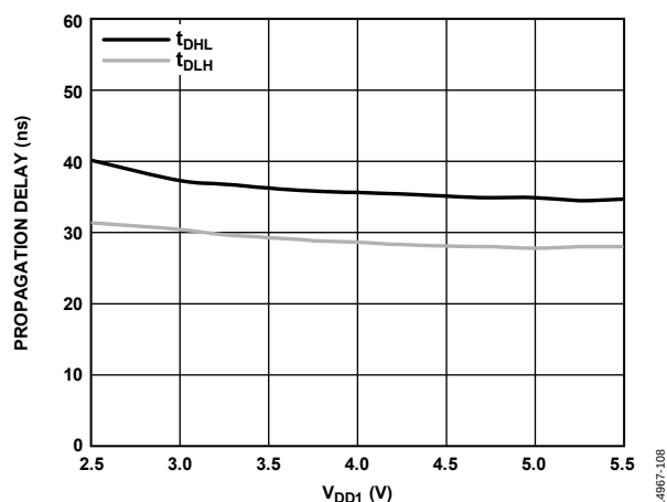
Figure 13. Propagation Delay vs. V_{DD1} , V_{DD2} = 15 V, 2 nF Load, 0 \Omega Gate Resistor
