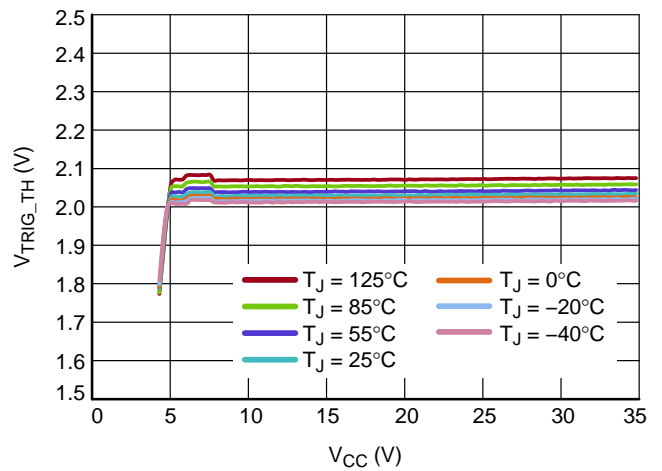
Figure 26. Trigger Threshold
