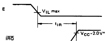
Figure 7 \overline{IRO} Release Time
