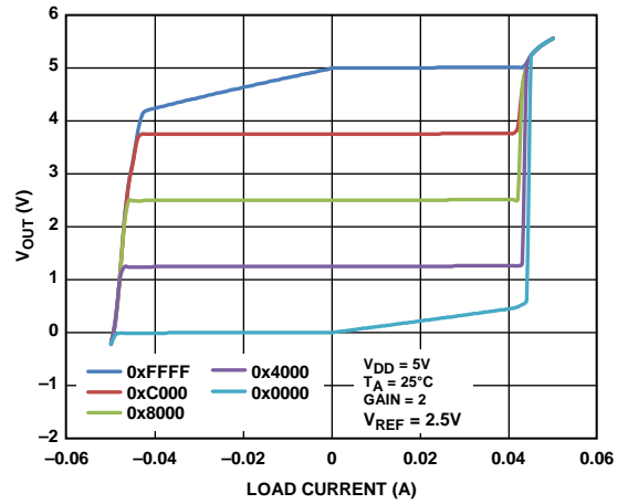
Figure 23. Source and Sink Capability at 5 V
