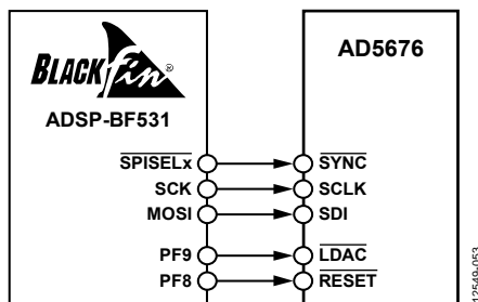
Figure 49. ADSP-BF531 Interface
