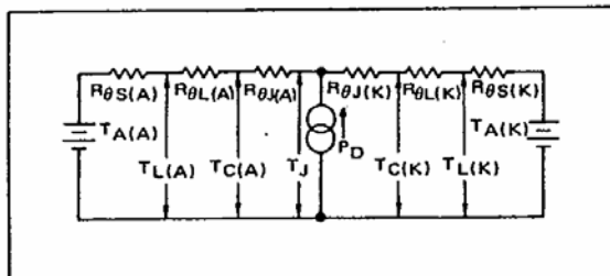
NOTE 3 -- APPROXIMATE THERMAL CIRCUIT MODEL
