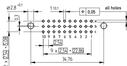
PCB drillhole pattern
