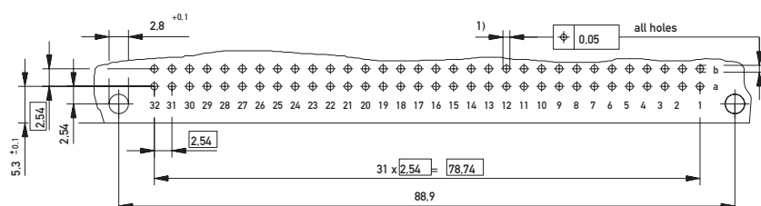
PCB drillhole pattern
