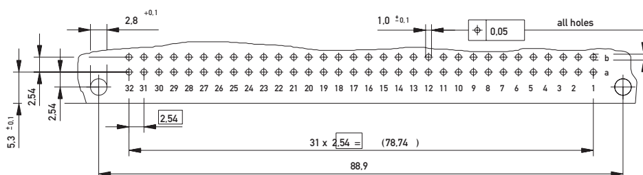
PCB drillhole pattern
