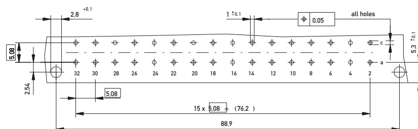
PCB drillhole pattern
