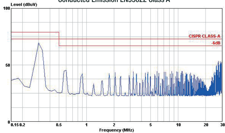
Conducted Emission EN55022 Class A
