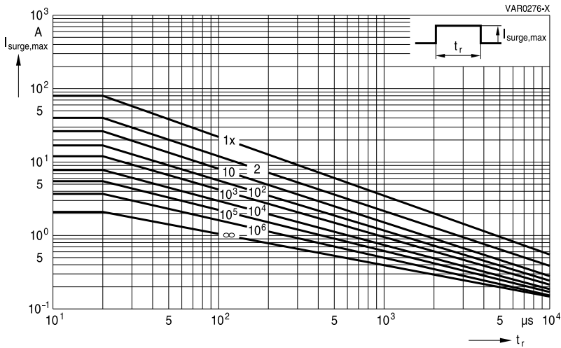
CT0805K20G ... K30G
