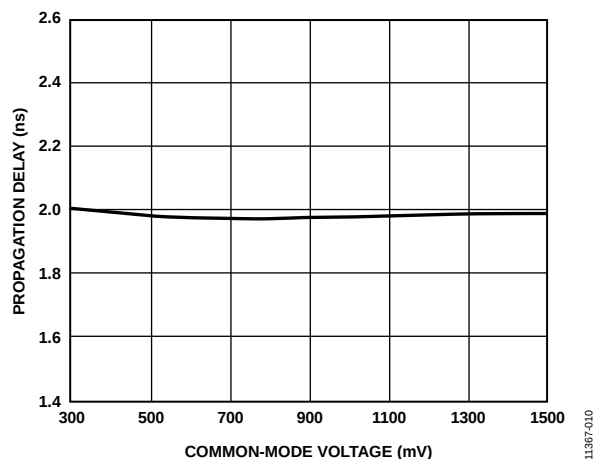
Figure 9. LVDS Propagation Delay vs. Input Common-Mode Voltage
