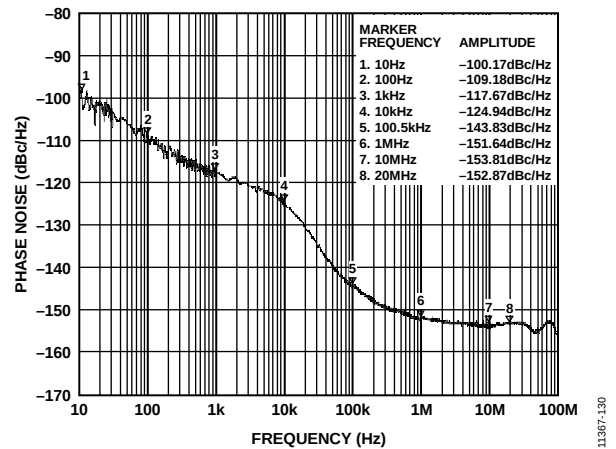
Figure 32. Additive Phase Noise with Clock Input = 622.08 MHz and LVDS Outputs = 622.08 MHz
