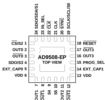
Figure 2. Pin Configuration
