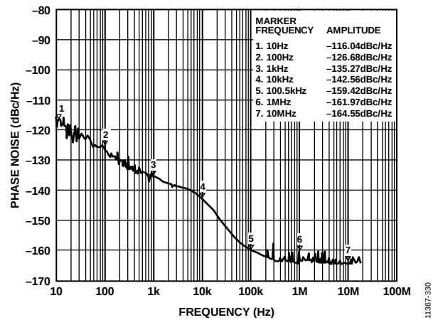
Figure 30. Additive Phase Noise with Clock Input = 1200 MHz and HSTL Outputs = 100 MHz
