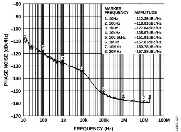
Figure 31. Additive Phase Noise with Clock Input = 622.08 MHz and HSTL Outputs = 155.52 MHz
