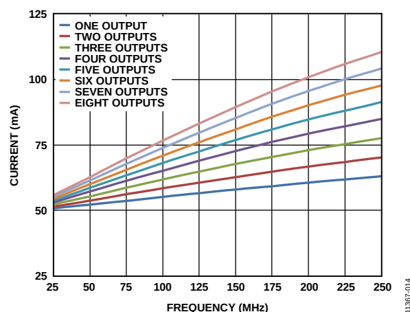
Figure 13. Power Supply Current vs. Frequency and Number of Outputs Used, CMOS Mode
