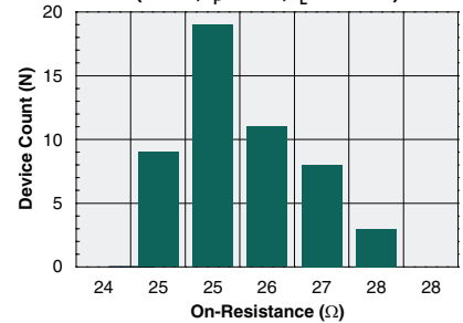
Typical On-Resistance Distribution (N=50, I_F=0mA , I_L=100mA )
