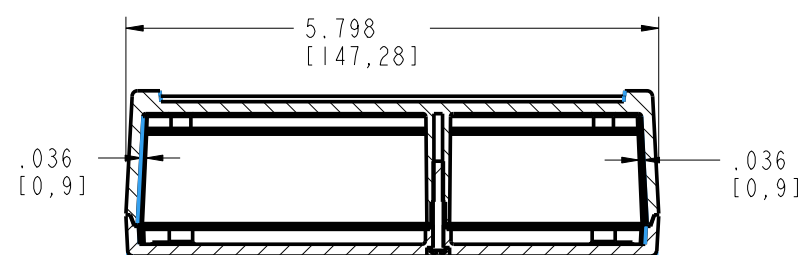
SECTION B-B ROTATED 90° CCW
