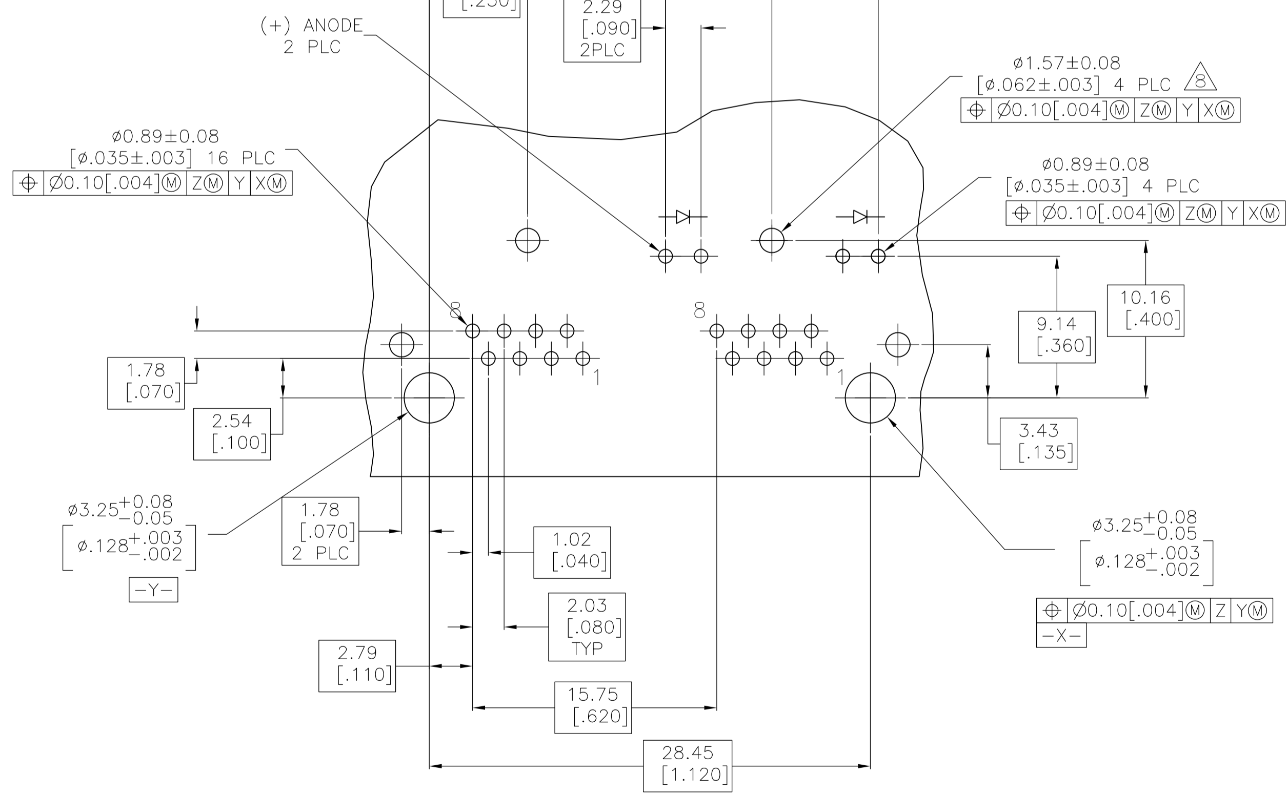
RECOMMENDED PRINTED CIRCUIT BOARD LAYOUT COMPONENT SIDE
